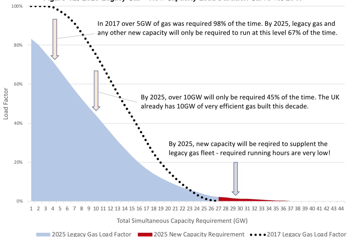
Figure 12. 2025 Legacy Gas + New Capacity Load Duration Curve vs. 2017
