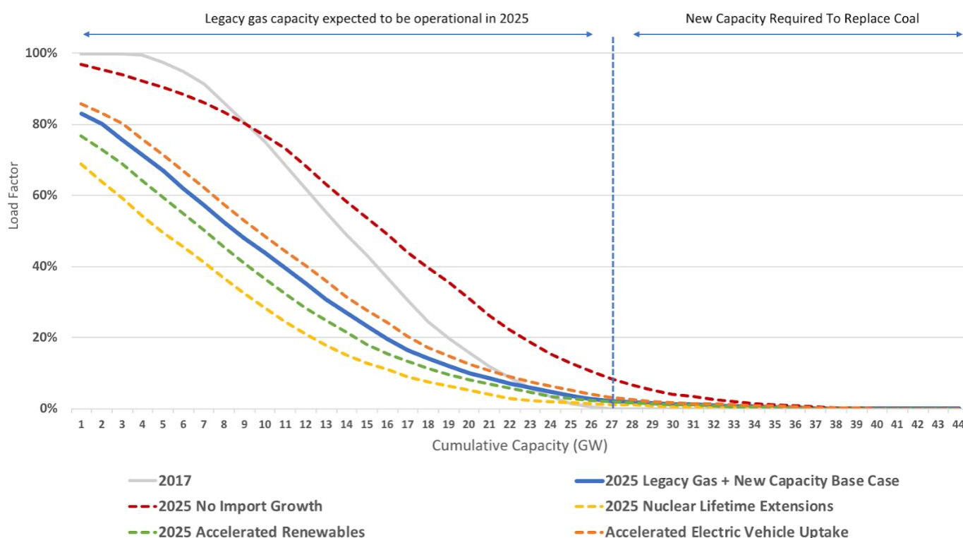
Figure 13. Scenario Analysis for 2025 Legacy Gas & New Capacity Load Duration Curves
