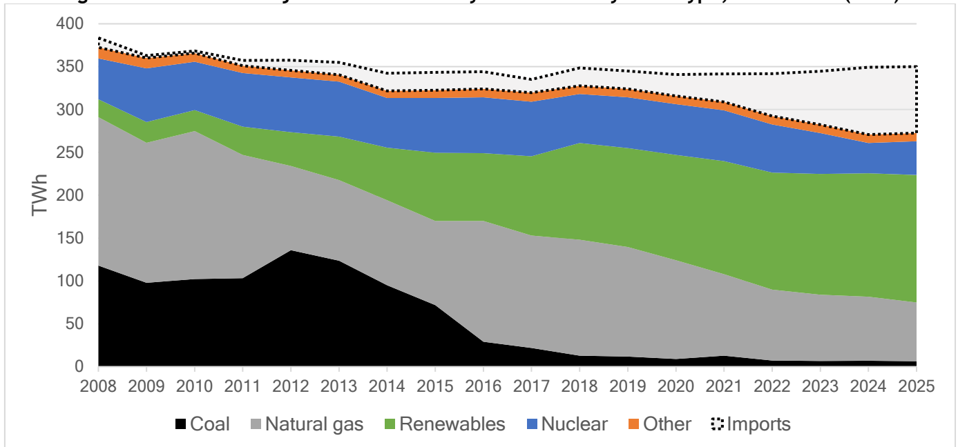
Figure 9. Historic & Projected UK Electricity Generation by Fuel Type, 2008-2025 (TWh)
