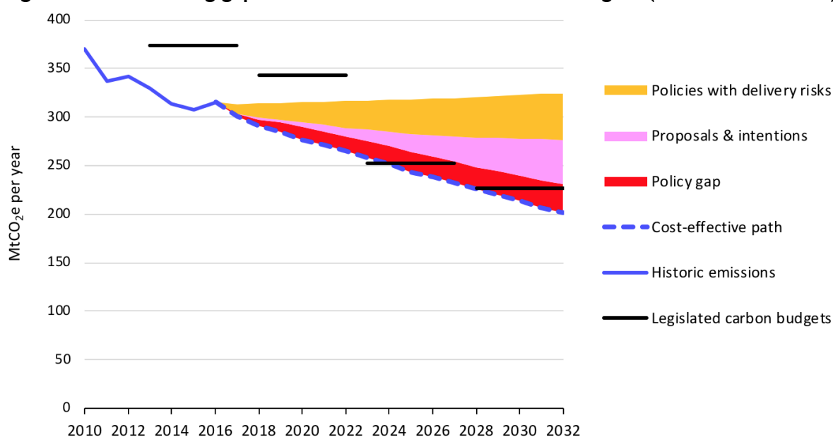
Figure 10. Remaining gaps to the fourth and fifth carbon budgets (non-traded sector)
