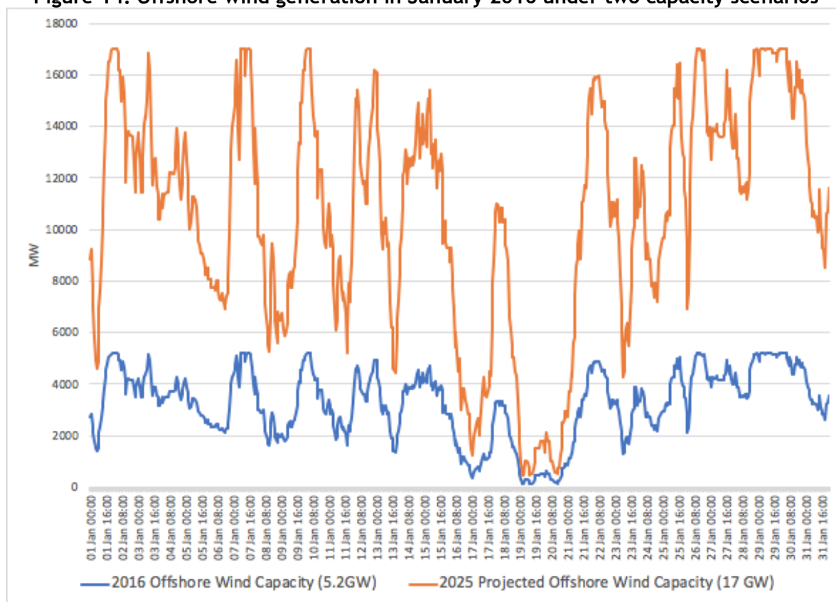
Figure 14. Offshore wind generation in January 2016 under two capacity scenarios
